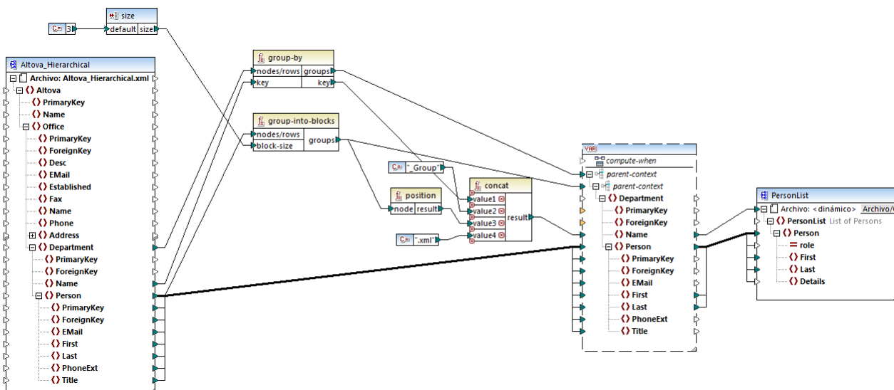
DividePersonsByDepartmentIntoGroups.mfd
