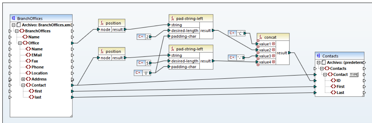
ContactsFromBranchOffices.mfd
