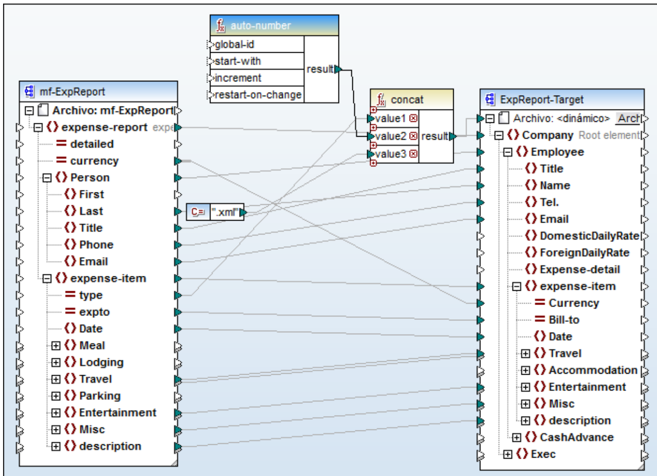
Tut-ExpReport-dyn.mfd (MapForce Basic Edition)
