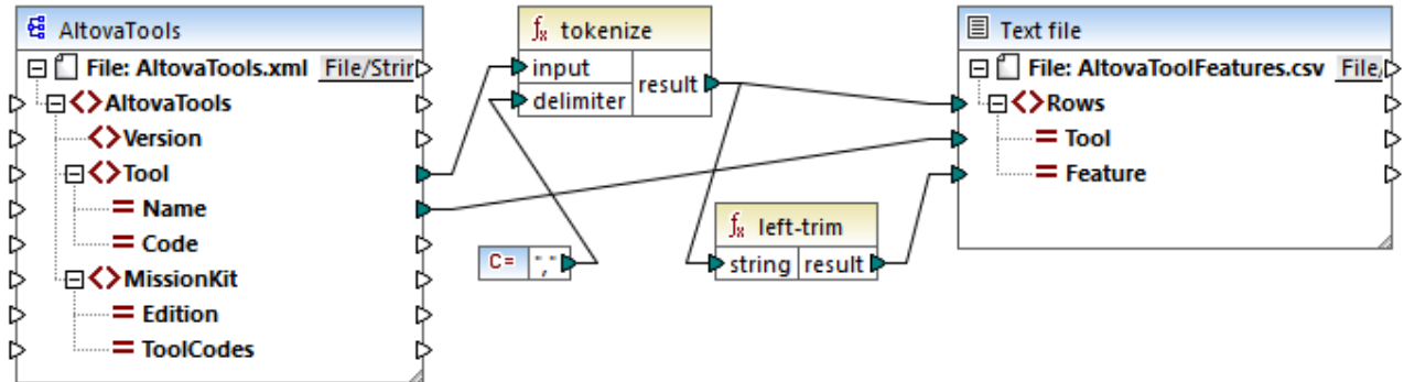
tokenizeString1.mfd
