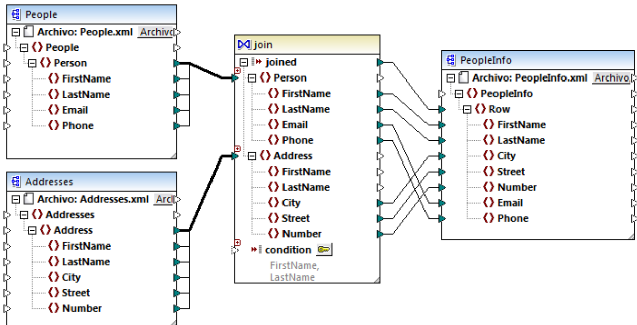
JoinPeopleInfo.mfd
