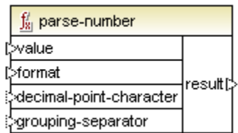
parse-number
