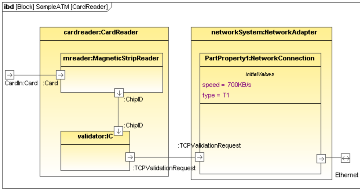
Diagrama CardReader
